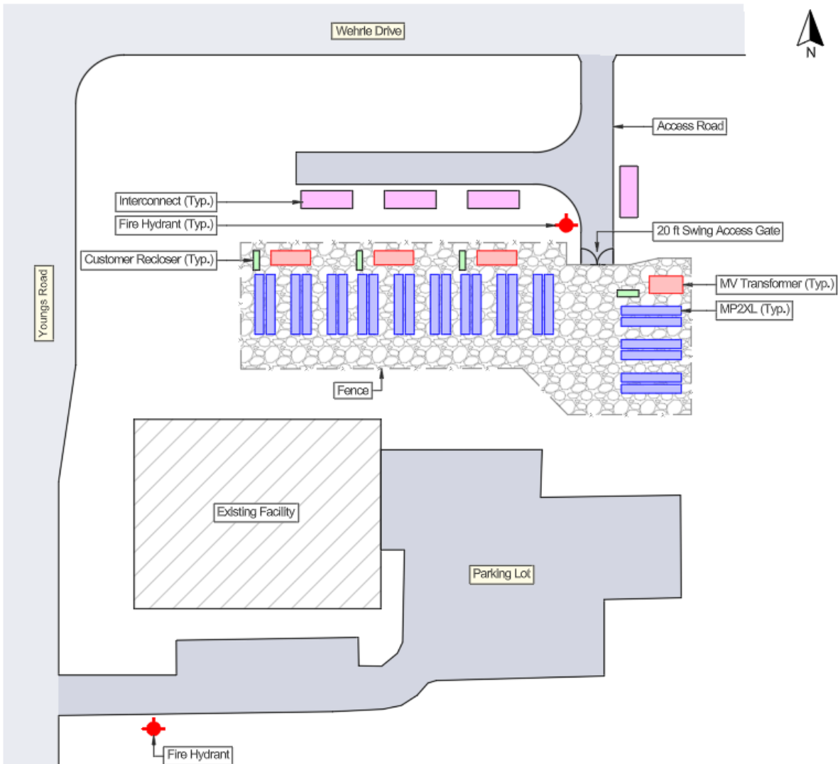
Figure 2: Renaissance BESS Facility Overview
