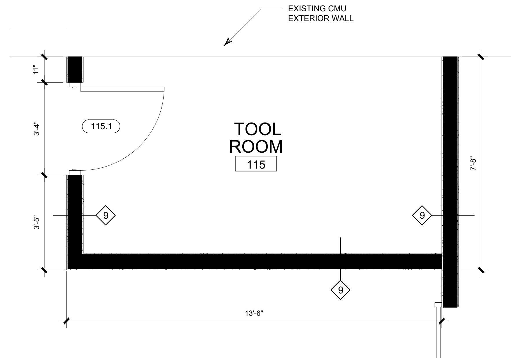
ENLARGED TOOL ROOM PLAN
