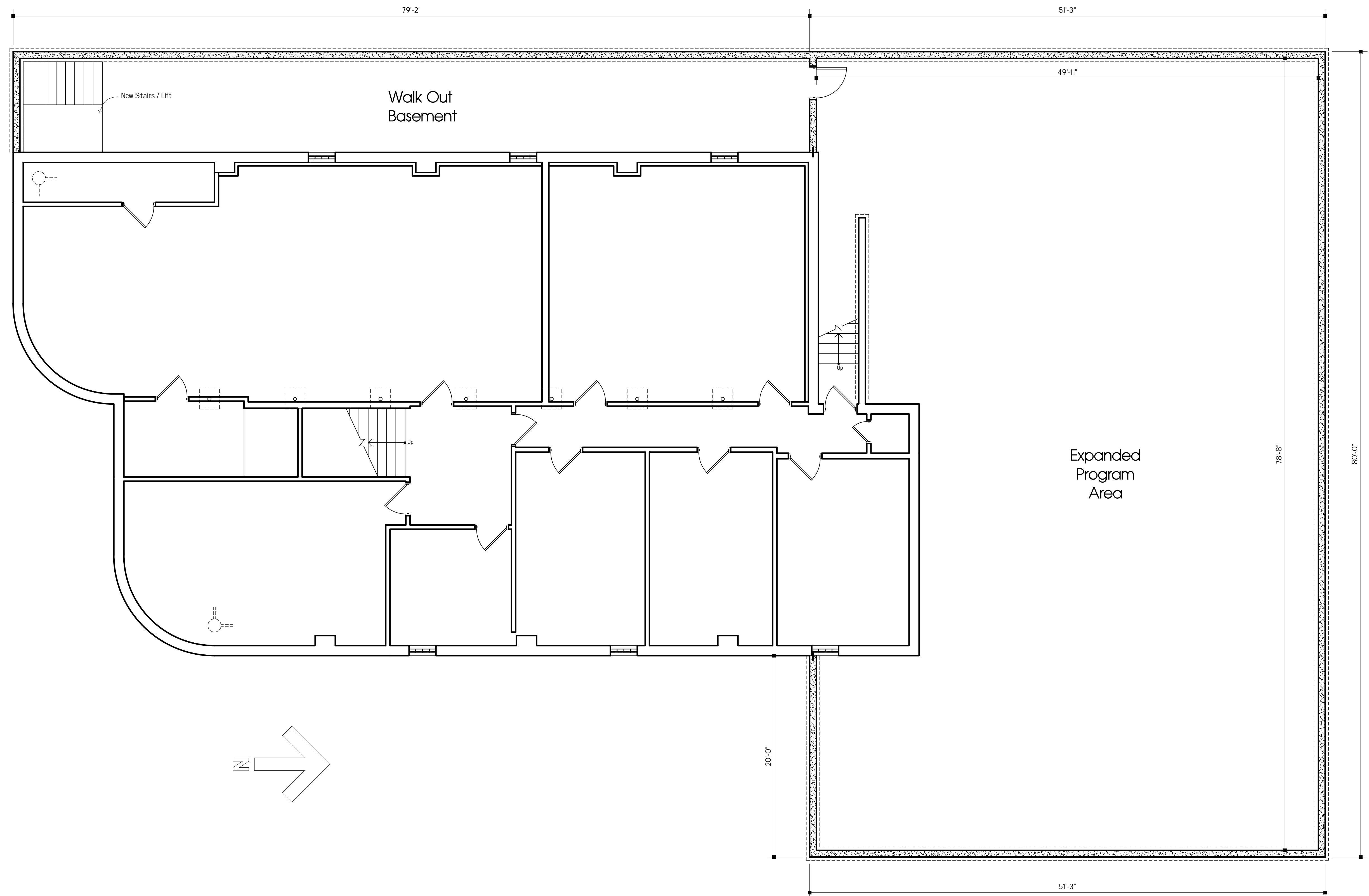
A2.1 Basement Concept Plan
