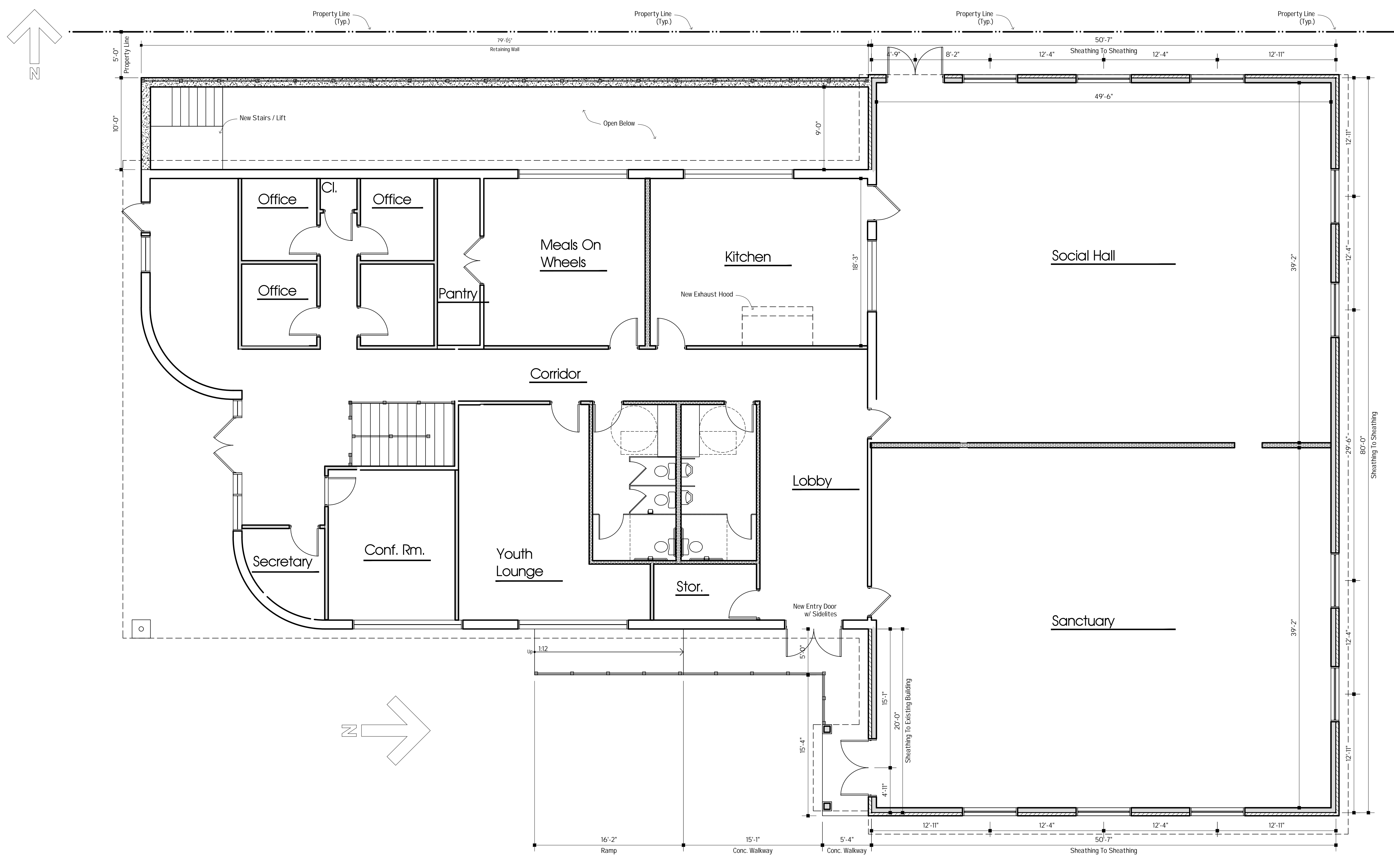
A1.1 First Floor Concept Plan
