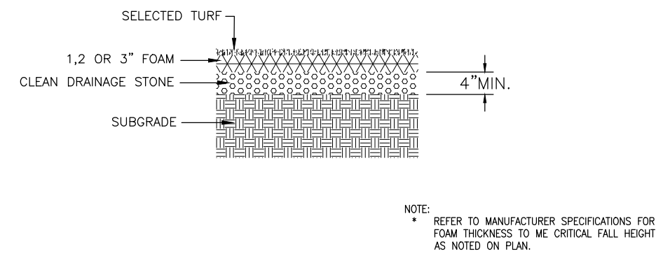
3 TURF SURFACING SCALE IN FEET: 1/2" = 1'-0"
