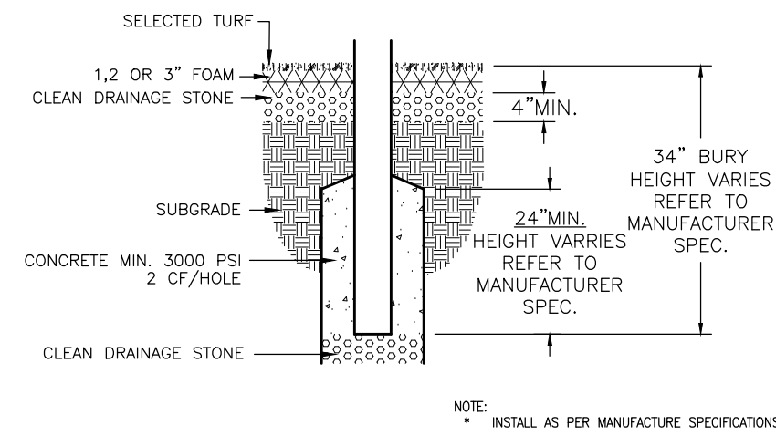
1 TYPICAL POST DETAIL - TURF SCALE IN FEET: 1/2" = 1'-0"
