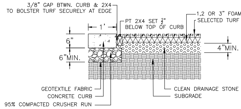
2 TURF SURFACING WITH CONCRETE BORDER SCALE IN FEET: 1/2" = 1'-0"
