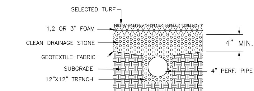
4 TURF DRAINAGE SECTION SCALE IN FEET: 1/2" = 1'-0"
