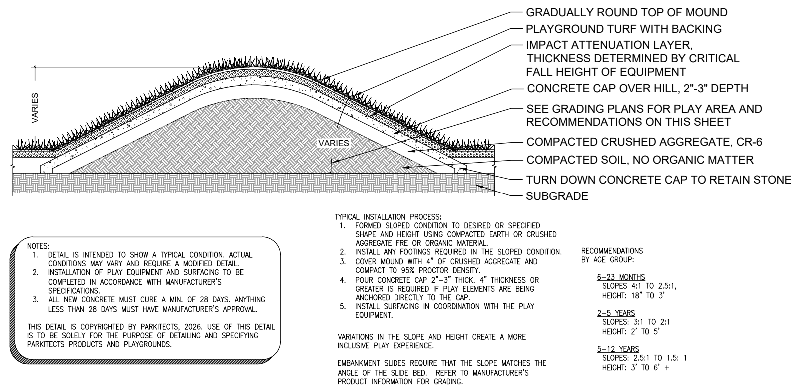
5 TYPICAL TURF SURFACING ON MOUND SCALE IN FEET: 1/2" = 1'-0"
