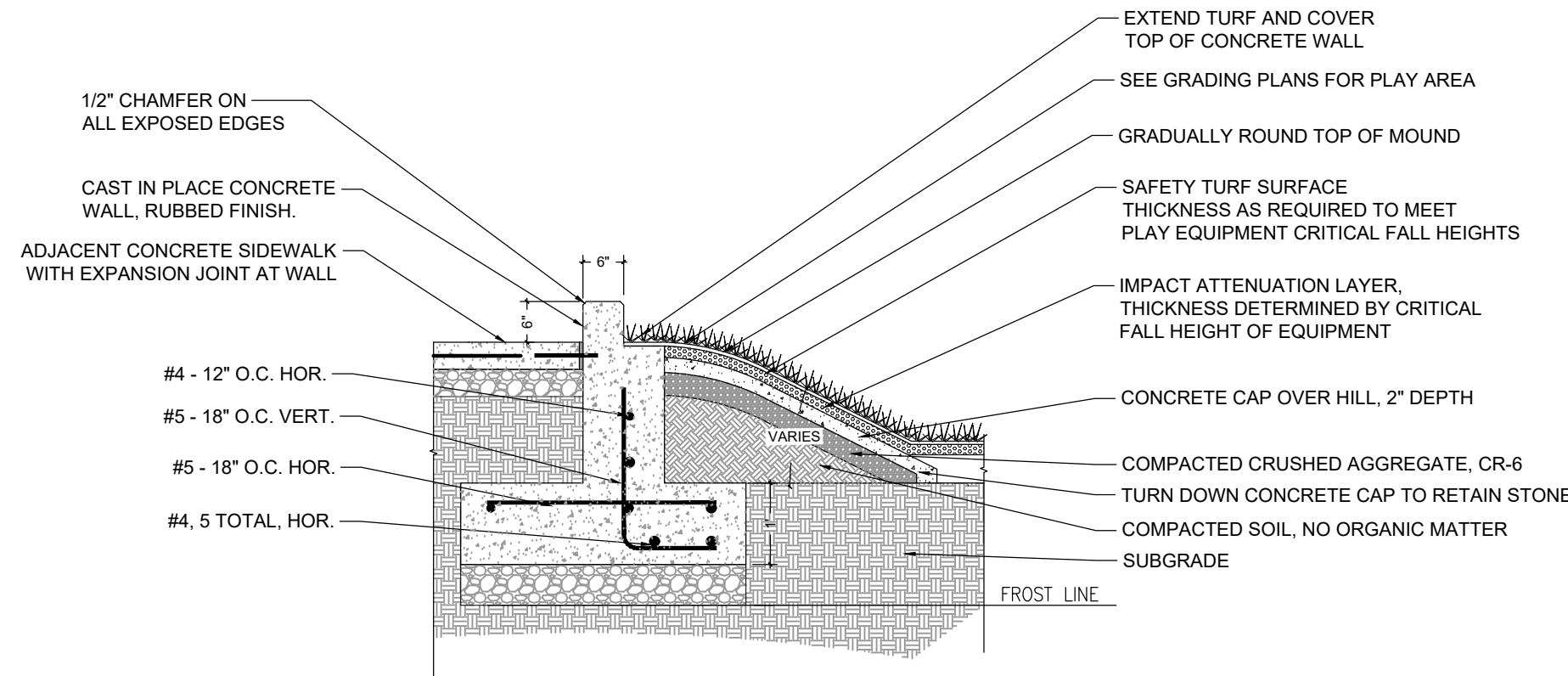
6 SECTION THROUGH ELEVATED PLAZA WITH WALL AND TURF SLOPE SCALE IN FEET: 1/2" = 1'-0"
